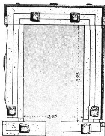
Εικ. 117. Τὸ θύρωμα τοῦ ἐν Νάξῳ ναοῦ τοῦ Διονύσου. (Welter)
