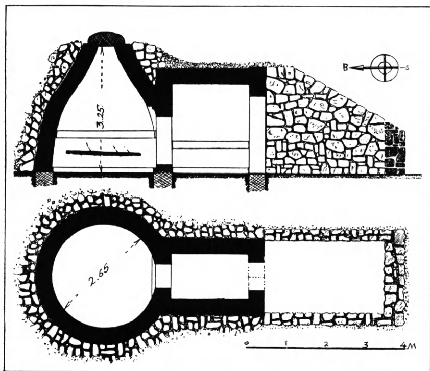
Εἰκ. 404. Κάτοψις καὶ κατὰ μῆκος τομὴ τοῦ παρὰ τὸ Καζανλάκ τῆς Β. Θράκης ἐλληνικοῦ τάφου (Micoff).
