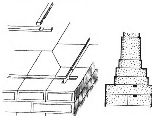
Εἰκ. 8. Αὐλακὲς πρὸς ἔνθεσιν σιδηρῶν ράβδων ἐκ τῆς κρηπίδος τοῦ ἐν Δελφοῖς θησαυροῦ τῶν Θηβαίων (Dinsmoor).
