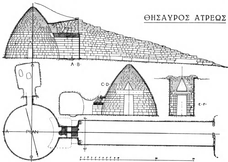
Εἰκ. 271. Ὅριζοντία καὶ κατακόρυφοι τομαὶ τοῦ ἐν Μυκῆναις θησαυροῦ τοῦ Ἀτρέως (Wace).
