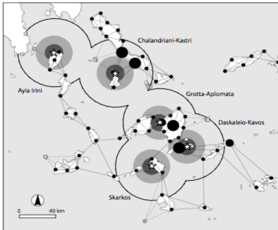
Fig. 2 One-day travel ranges from major Early Bronze II Cycladic centres, indicating several zones of interaction that differed in nature and intensity.
